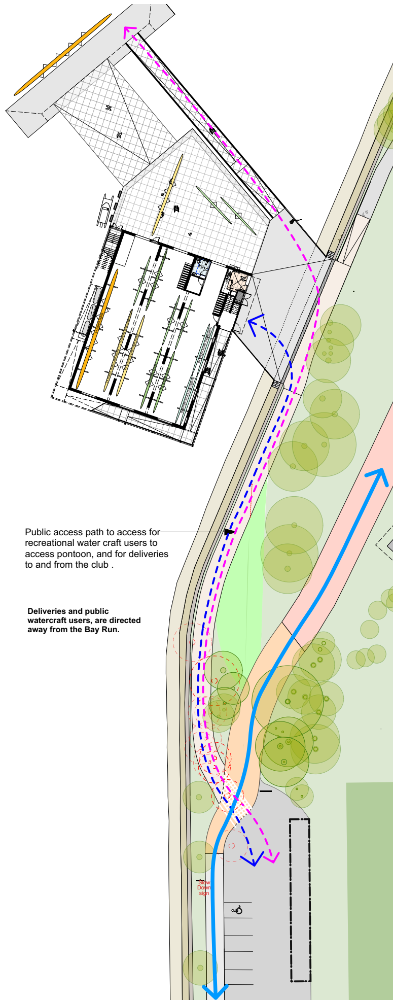
3. Deliveries and Public access to Pontoon
