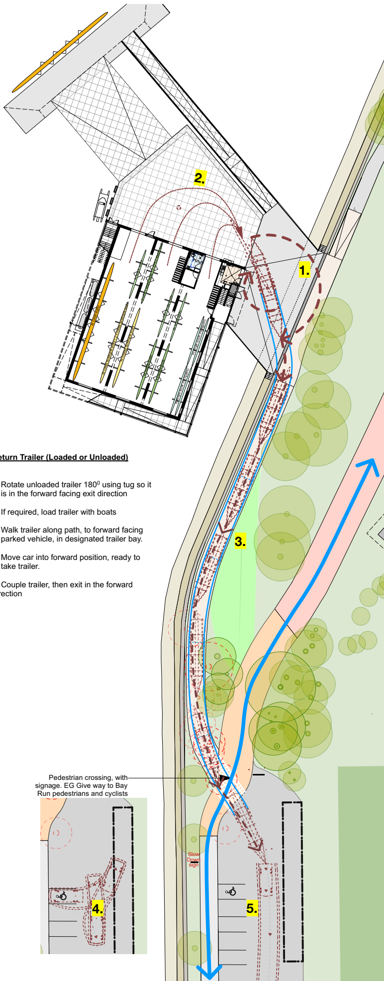
2. Bringing Trailer Back to vehicle (loaded or unloaded)
